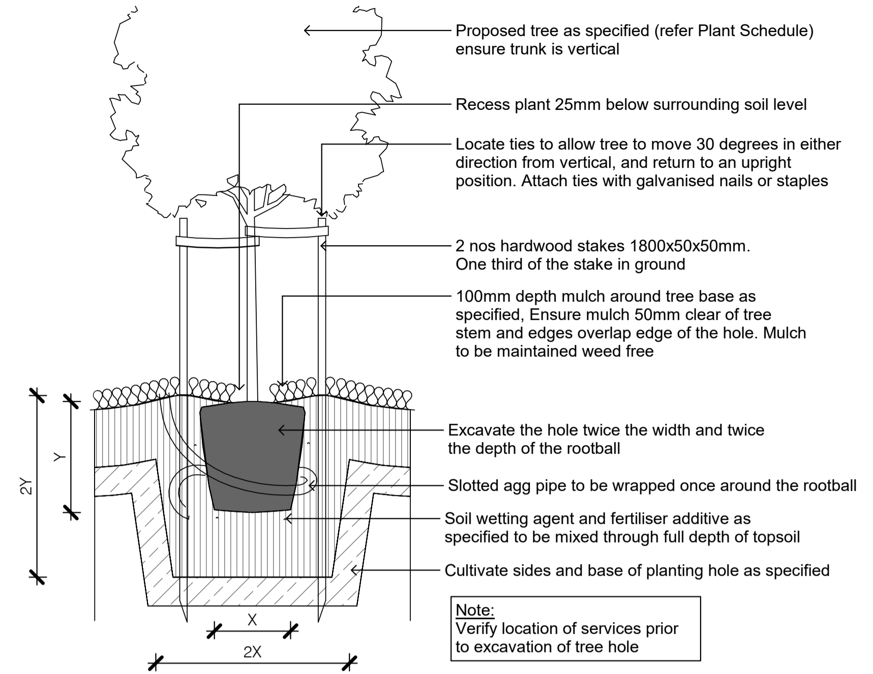
4 Typical Tree Planting SCALE - 1 : 20 @ A1
