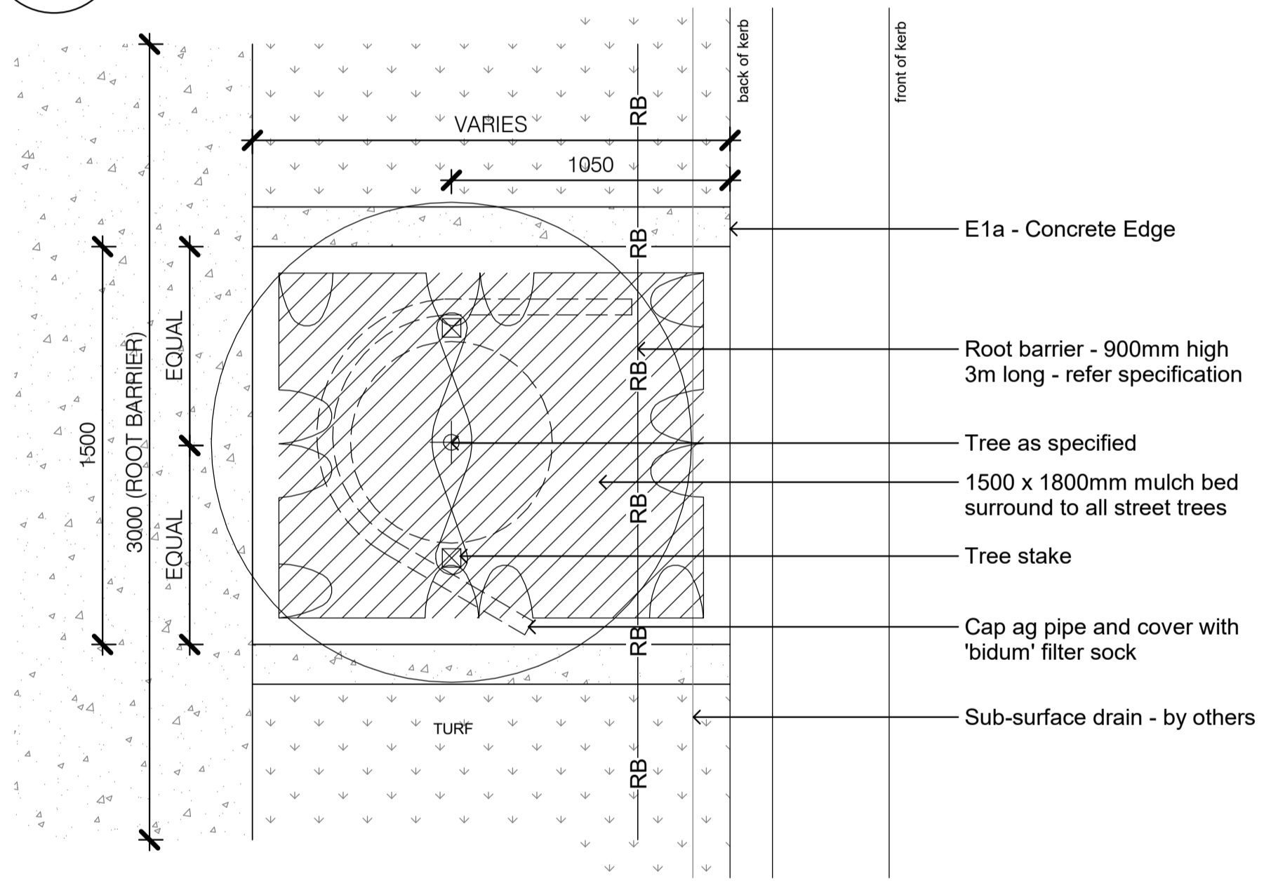
5 Boulevard Street Tree Planting - to back of kerb SCALE - 1 : 20 @ A1
