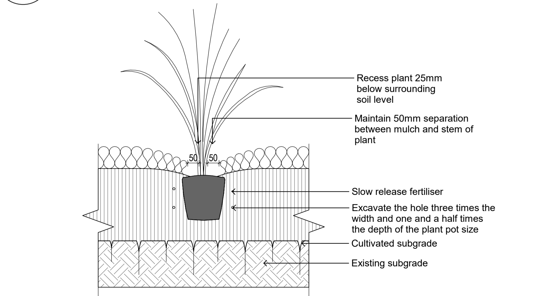
6 Typical Planting - 100mm to 300mm stock SCALE - 1 : 10 @ A1
