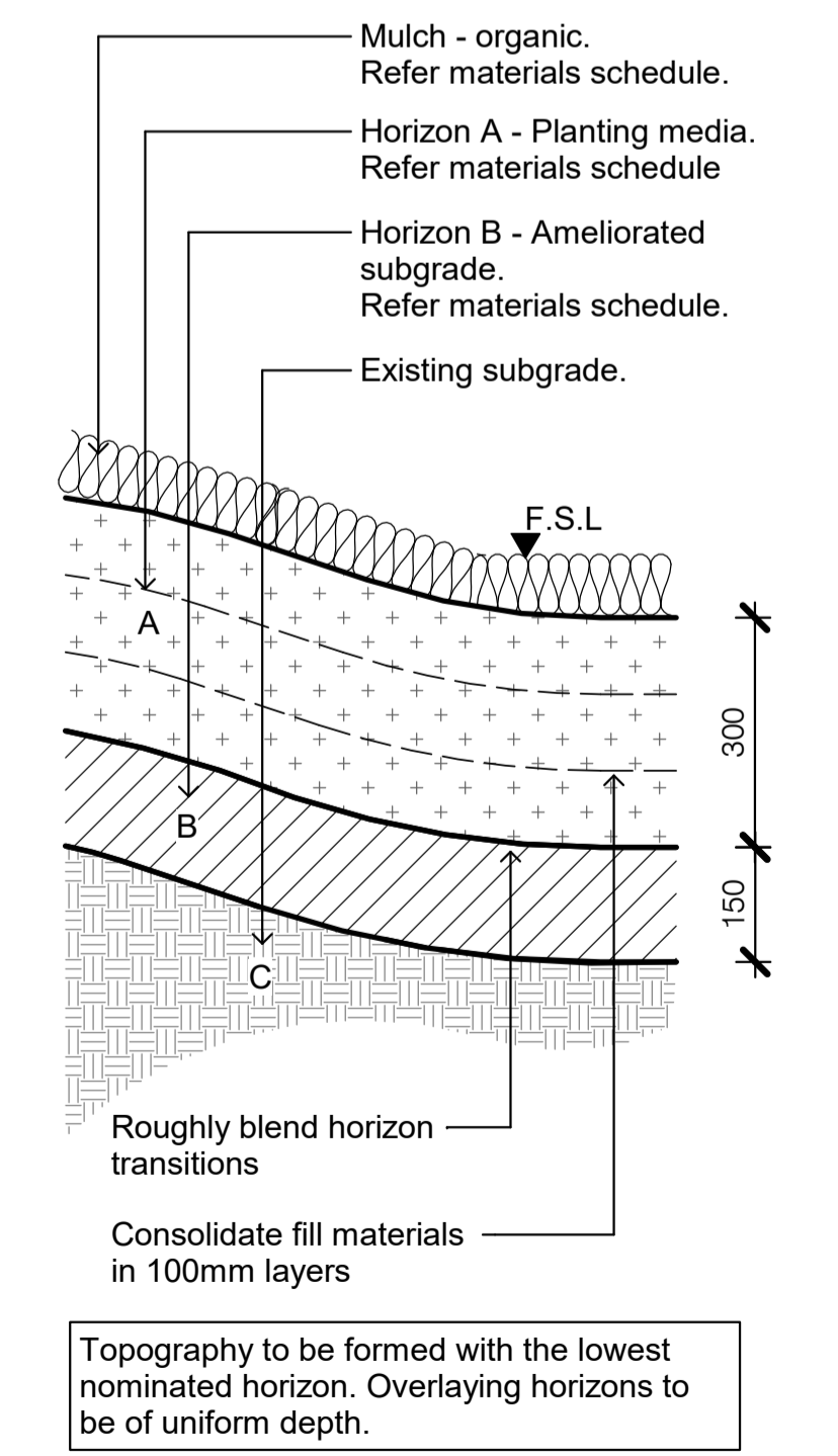
8 PA1 - Planting on Ground SCALE - 1 : 10 @ A1
