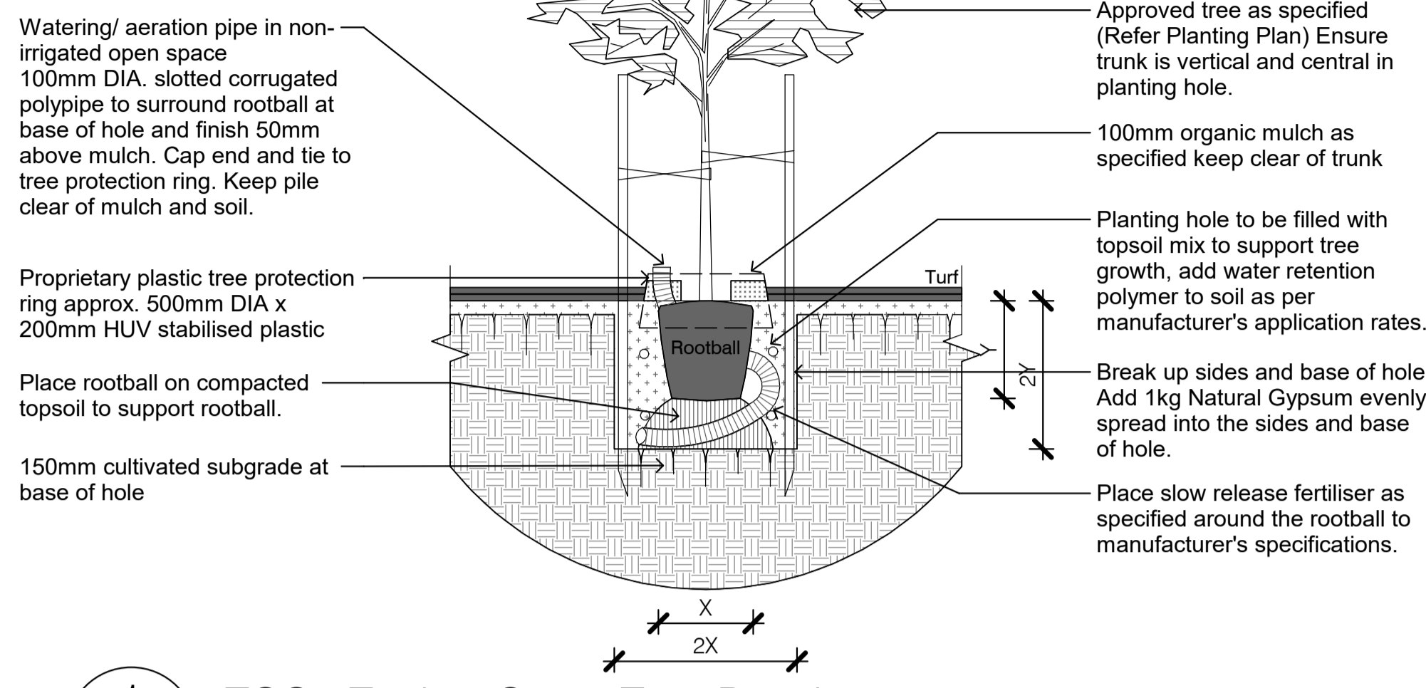
1 TCC - Typical Street Tree Planting SCALE - 1 : 20 @ A1
