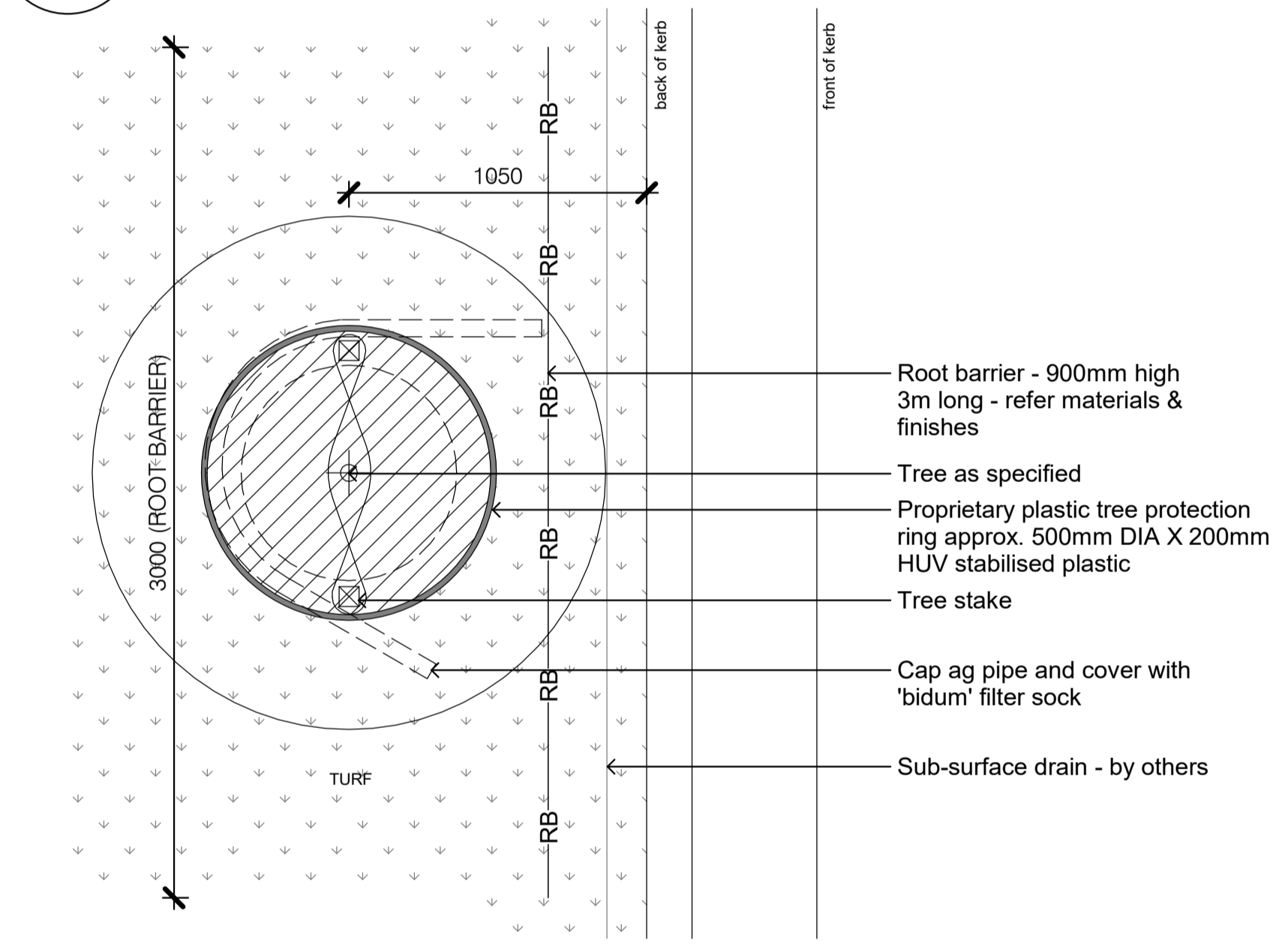
2 TCC - Typical Street Tree Planting - to back of kerb SCALE - 1 : 20 @ A1
