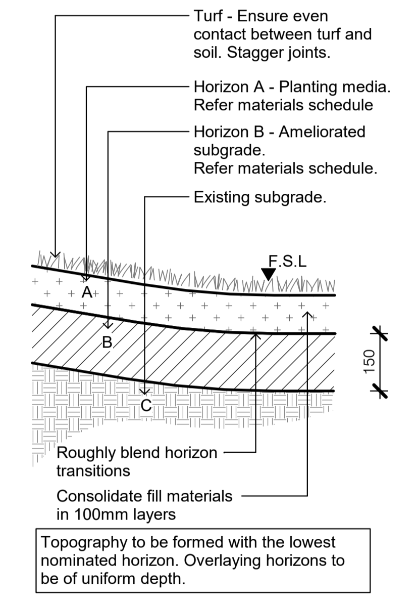
7 TF1 - Turf on Ground SCALE - 1 : 10 @ A1
