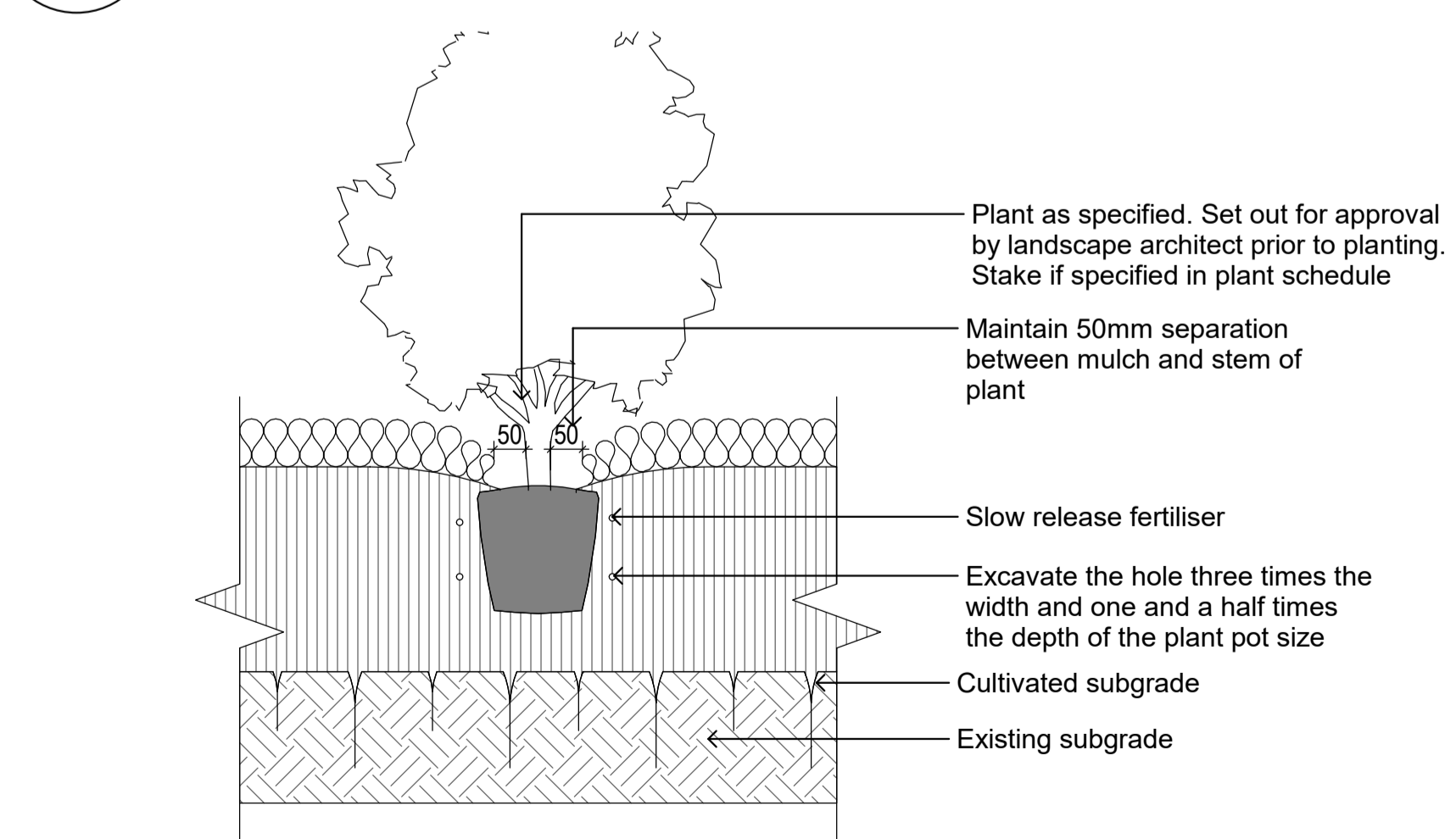
3 Typical Shrub / Groundcover Planting SCALE - 1 : 10 @ A1
